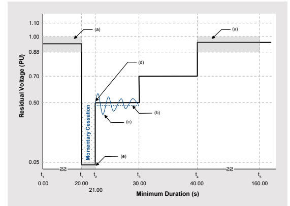
Figure 2 - LVRT as per 1547.1:2020 Section 5.4.4
